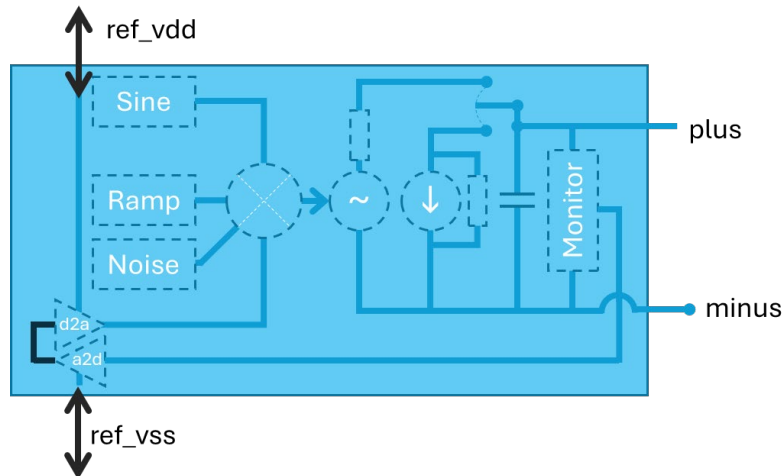
Figure 8: Mixed-signal bridge
