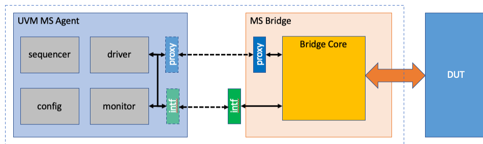
Figure 1: UVM-MS Architecture
