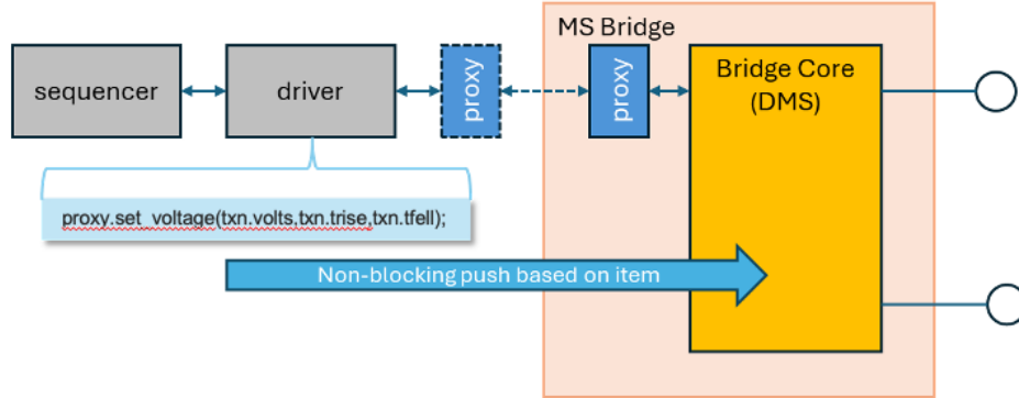
Figure 13: Push analog control – DMS version
