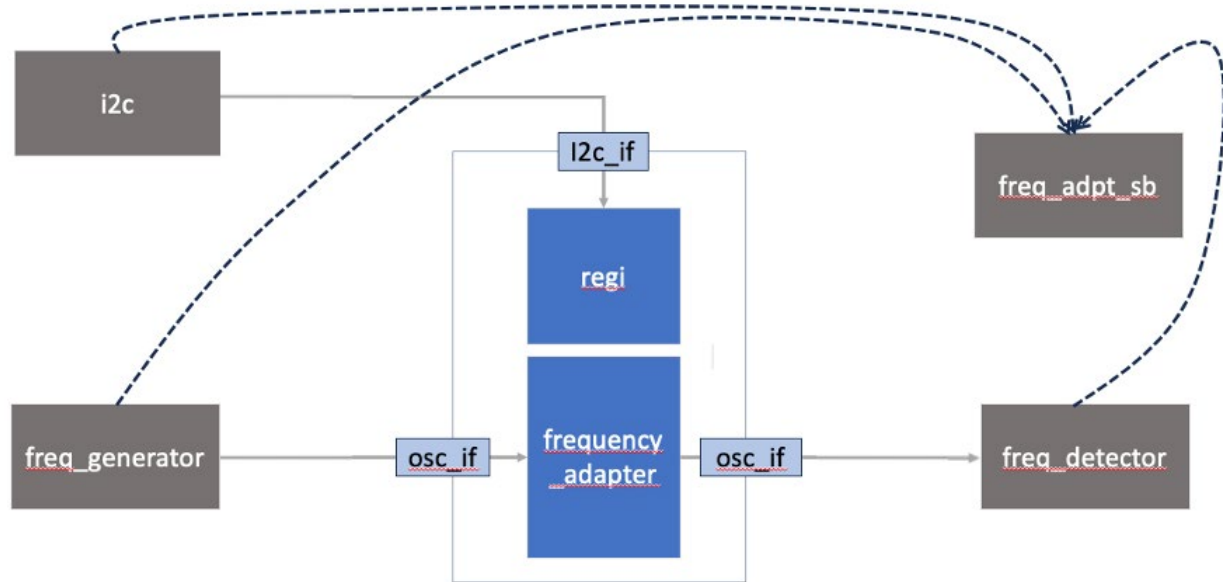
Figure 20: UVM testbench, showing oscillator interface
